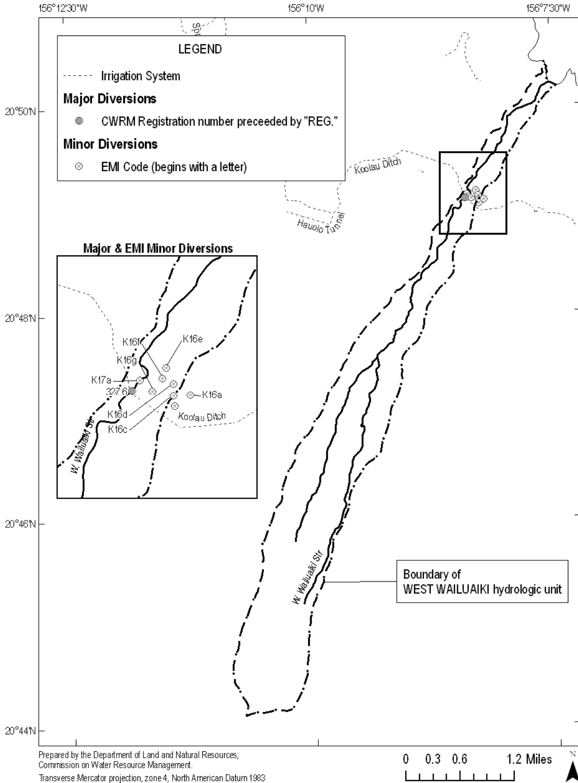
Figure 13-19. All registered diversions and EMI minor diversions identified in the West Wailuaiki hydrologic unit (Source: East Maui Irrigation Company, 1970; State of Hawaii, Commission on Water Resource Management, 2008f; USGS, 2001b).
