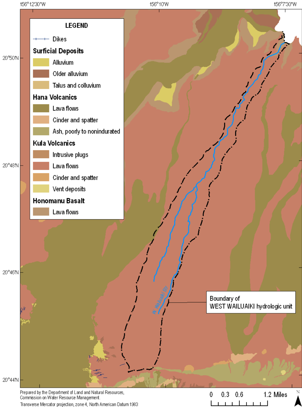
Figure 2-2. Generalized geology of West Wailuaiki hydrologic unit (Source: Sherrod et al., 2007; State of Hawaii, Office of Planning, 2006a, and State of Hawaii, Commission on Water Resource Management, 2008d; USGS, 2001b).
