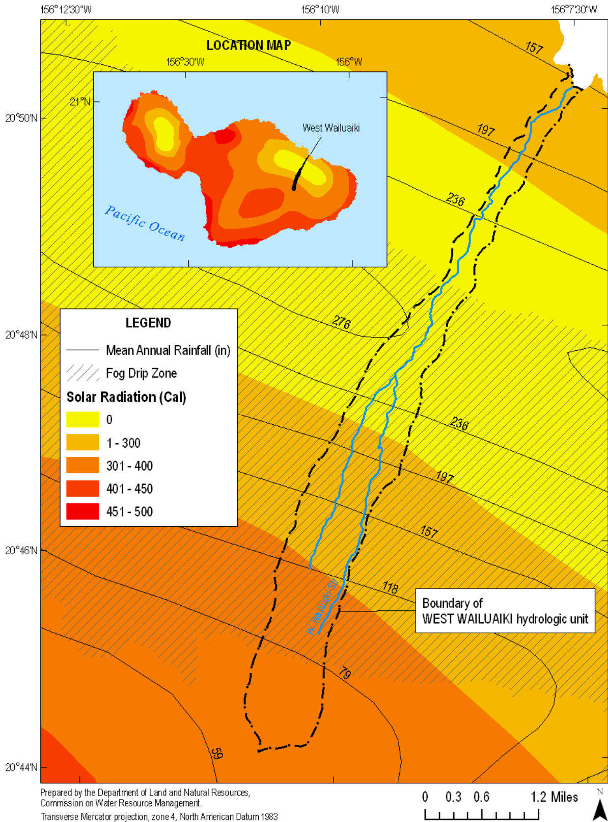
Figure 2-4. Mean annual rainfall and fog area in West Wailuaiki; and solar radiation for West Wailuaiki and the island of Maui, Hawaii (Source: Giambelluca et al., 1986; State of Hawaii, Office of Planning, 2006b; 2006c; USGS, 2001b).
