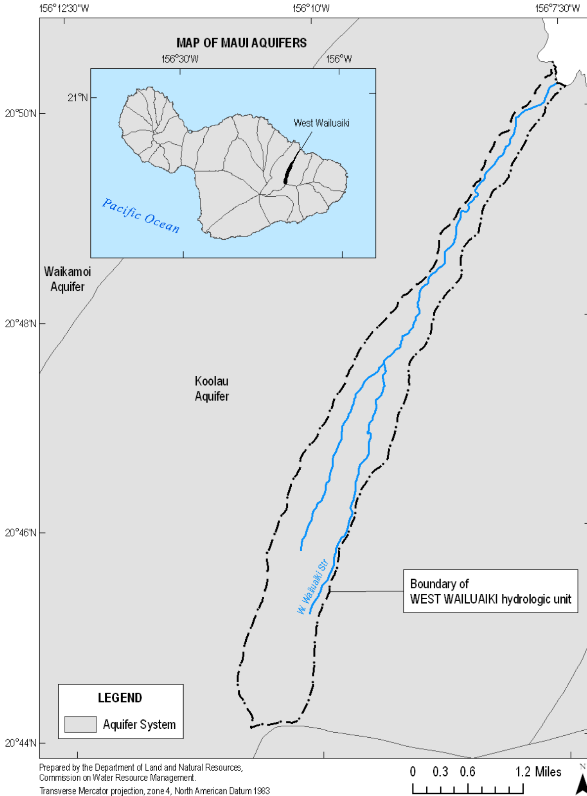
Figure 3-2. Aquifer system area and well locations in West Wailuaiki hydrologic unit (Source: State of Hawaii, Office of Planning, 2006b; State of Hawaii, Commission on Water Resource Management, 2008d; USGS 2001b).
