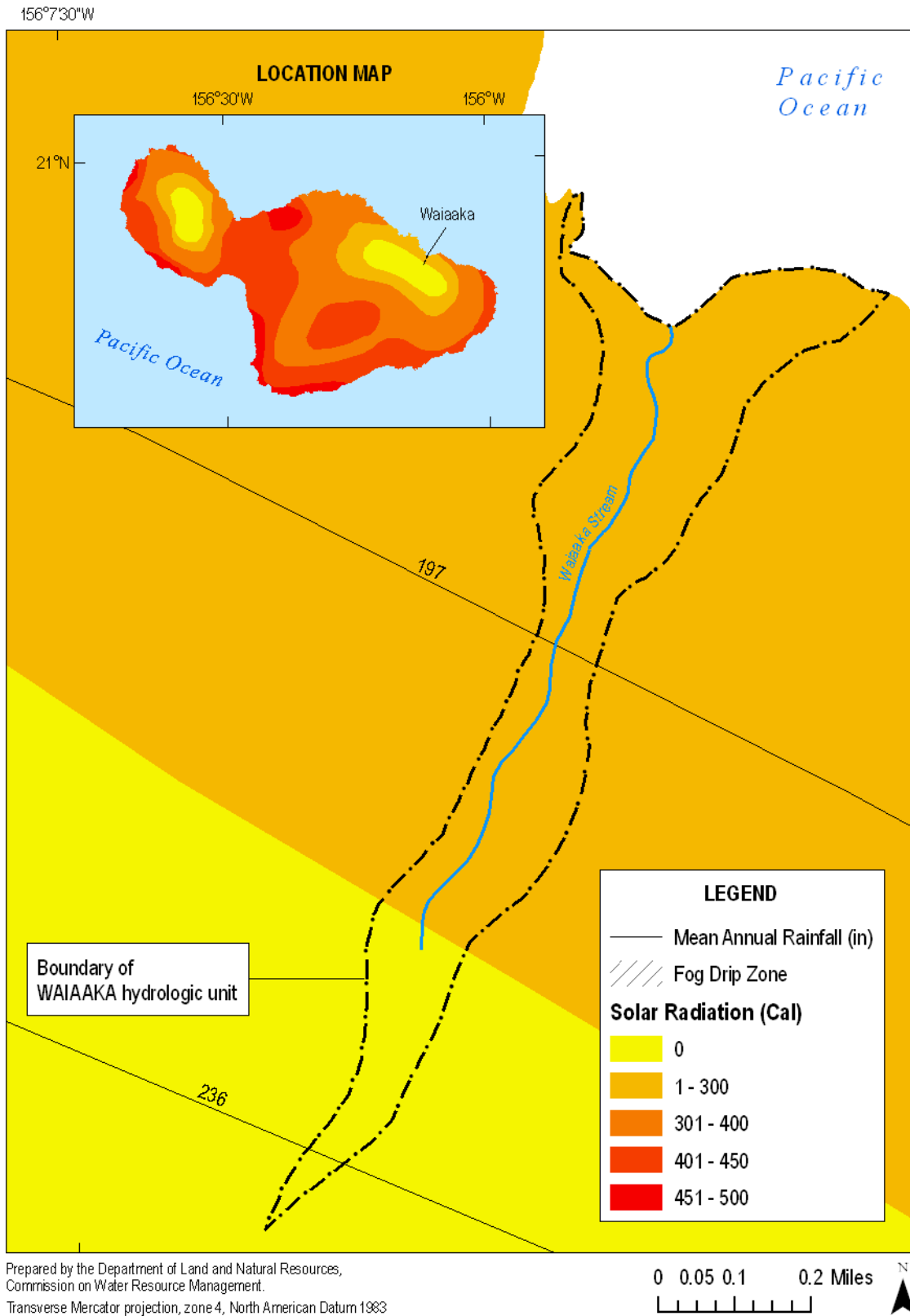
Figure 2-4. Mean annual rainfall and fog area in Waiaaka; and solar radiation for Waiaaka and the island of Maui, Hawaii (Source: Giambelluca et al., 1986; State of Hawaii, Office of Planning, 2006b; 2006c; USGS, 2001b).
