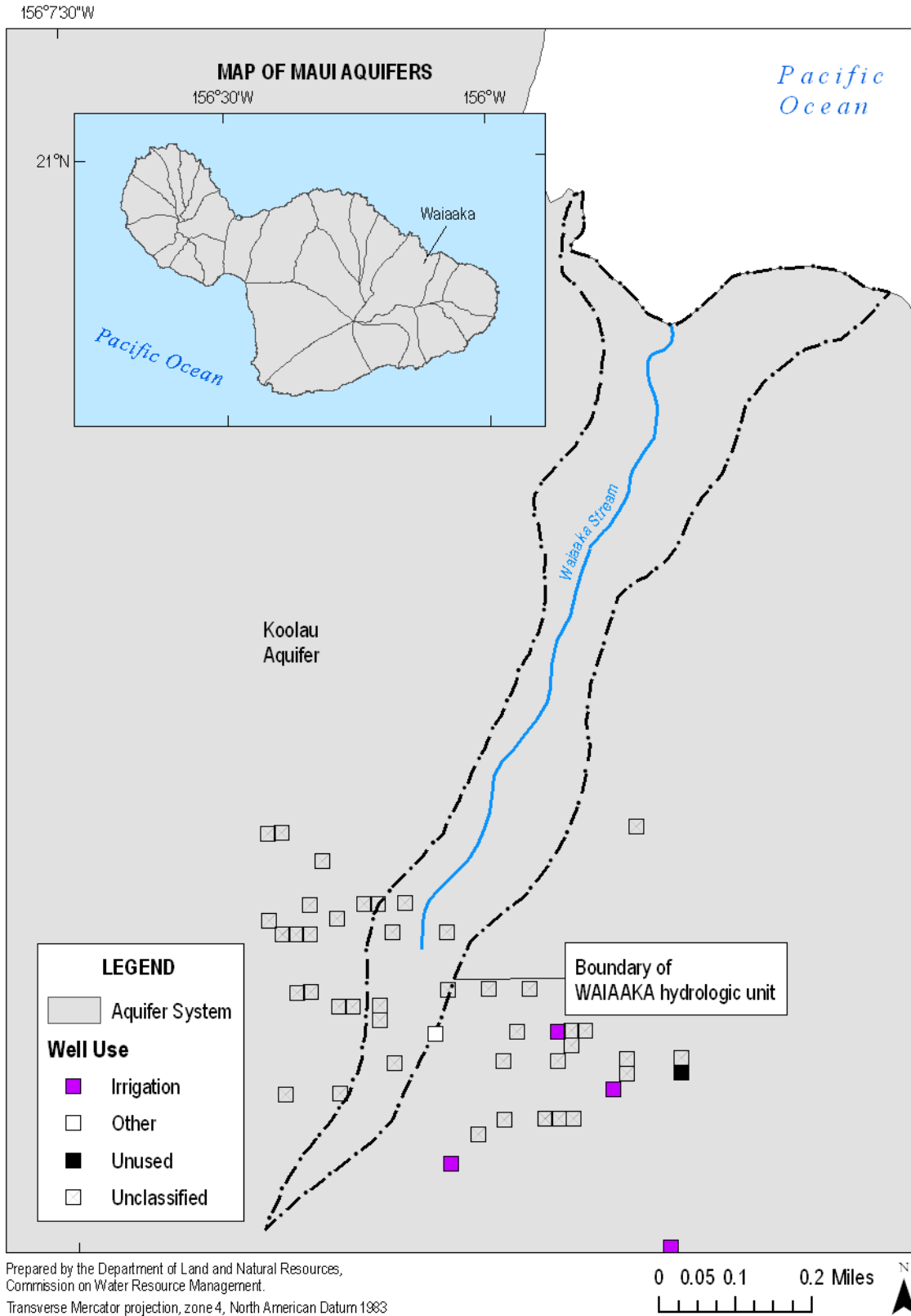
Figure 3-2. Aquifer system area and well locations in Waiaaka hydrologic unit (Source: State of Hawaii, Office of Planning, 2006b; State of Hawaii, Commission on Water Resource Management, 2008d; USGS, 2001b).
