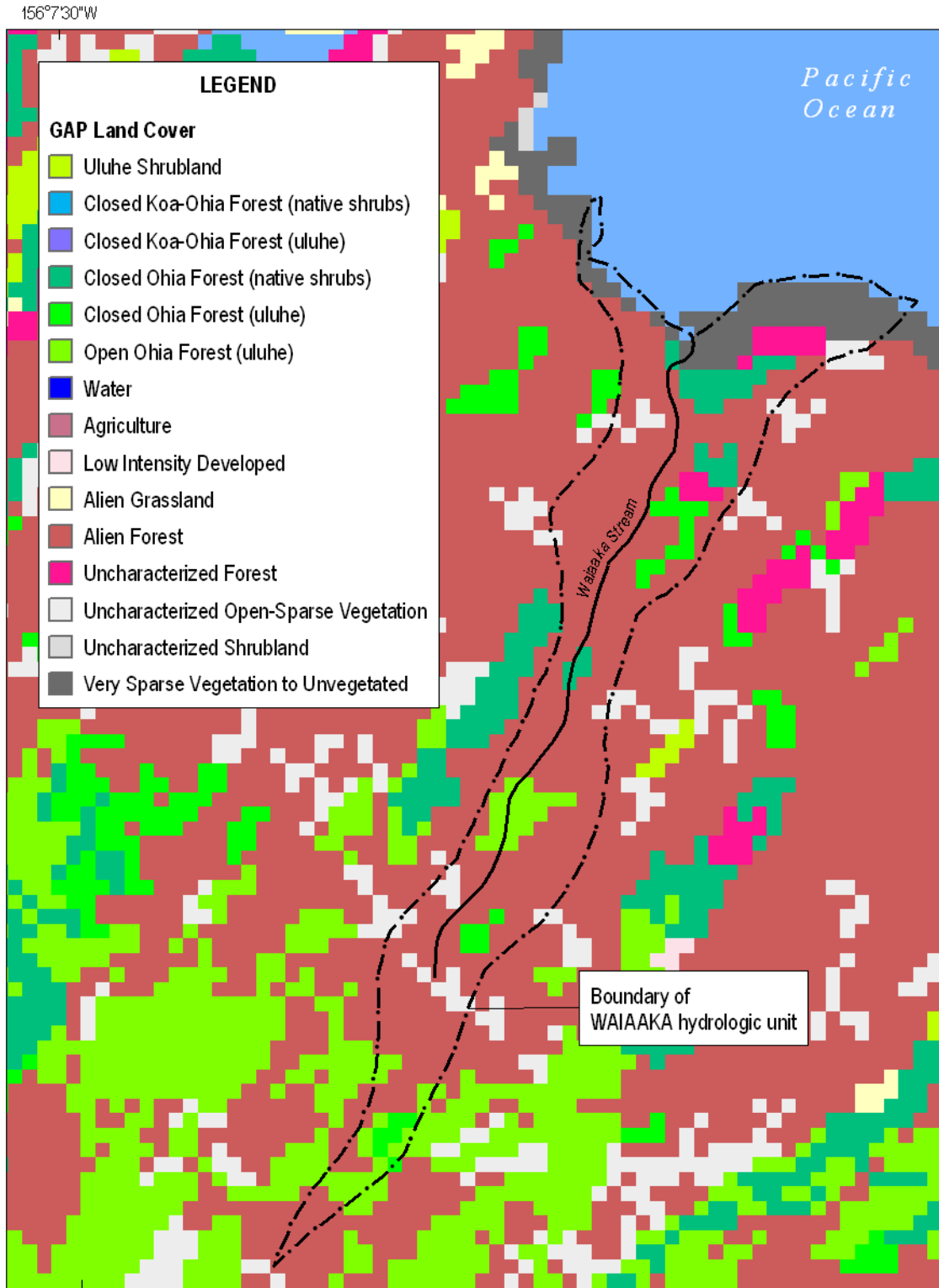
Figure 2-7. Hawaii GAP land cover classes in Waiiaka hydrologic unit (Source: Hawaii GAP Analysis Program, 2005; USGS, 2001b).
