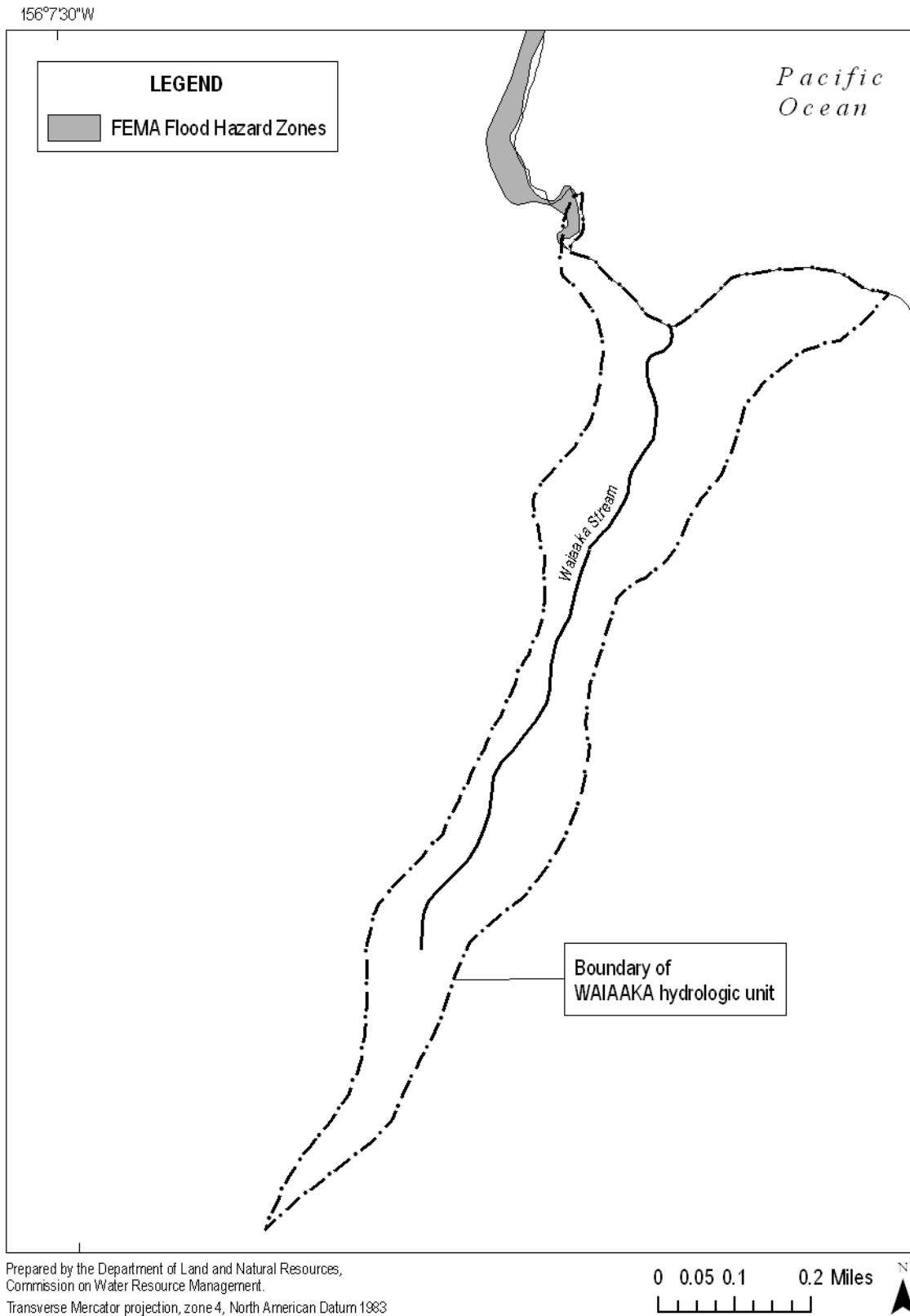
Figure 2-8. FEMA flood hazard zones in Waiiaka hydrologic unit (Source: Federal Emergency Management Agency, 2003; USGS, 2001b).
