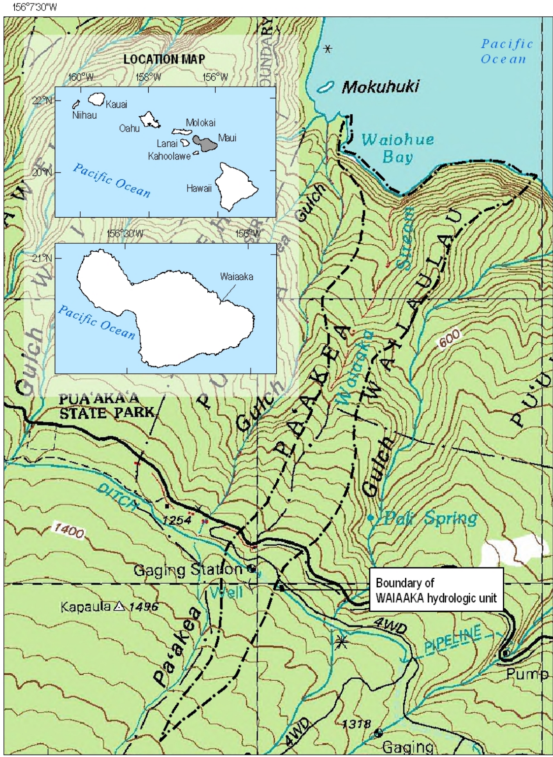
Figure 1-3. Topographic map of the Waiaka hydrologic unit in east Maui, Hawaii (Source: USGS, 1996).
