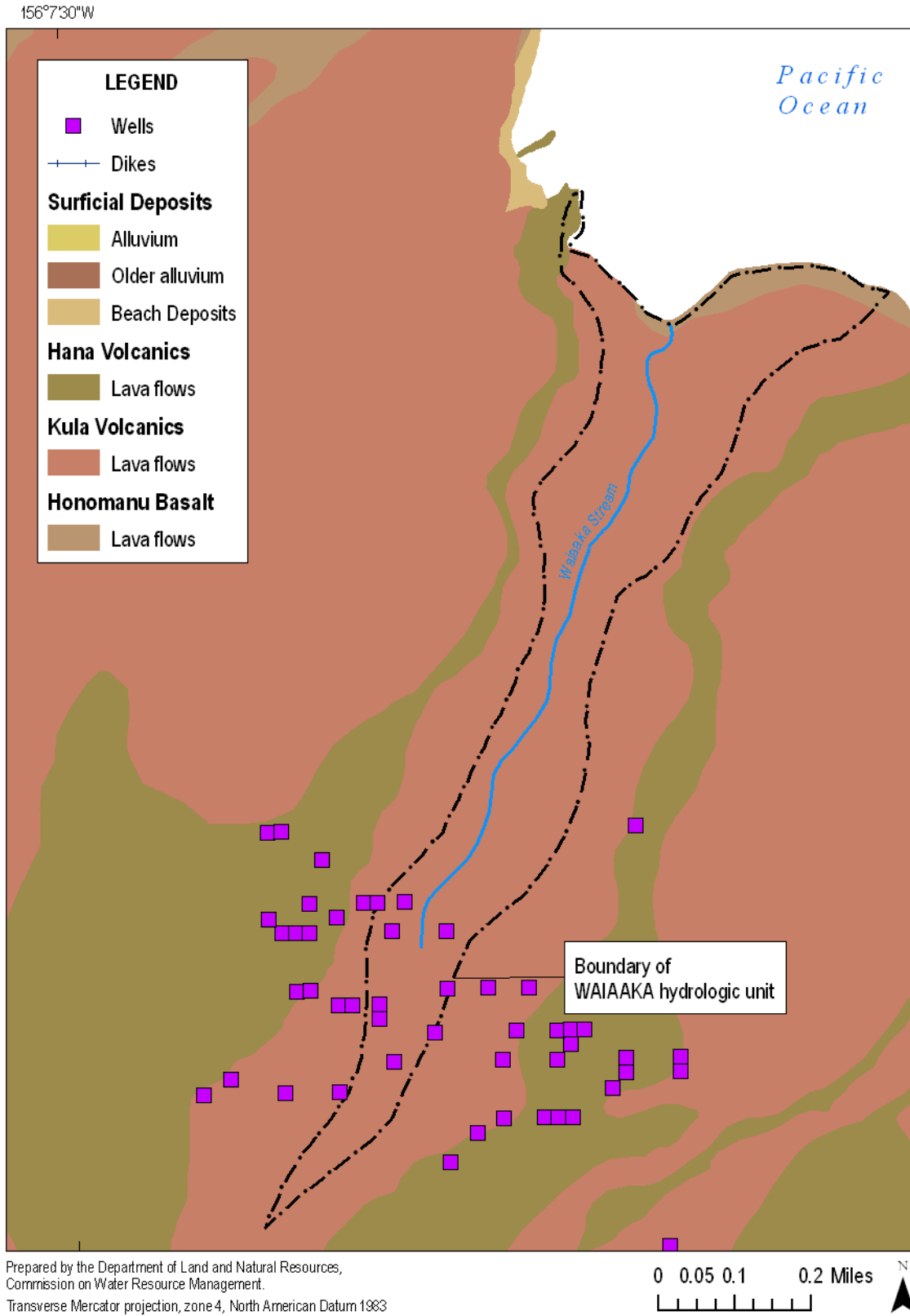
Figure 2-2. Generalized geology of Waiiaka hydrologic unit (Source: Sherrod et al., 2007; State of Hawaii, Office of Planning, 2006a, and State of Hawaii, Commission on Water Resource Management, 2008d; USGS, 2001b).
