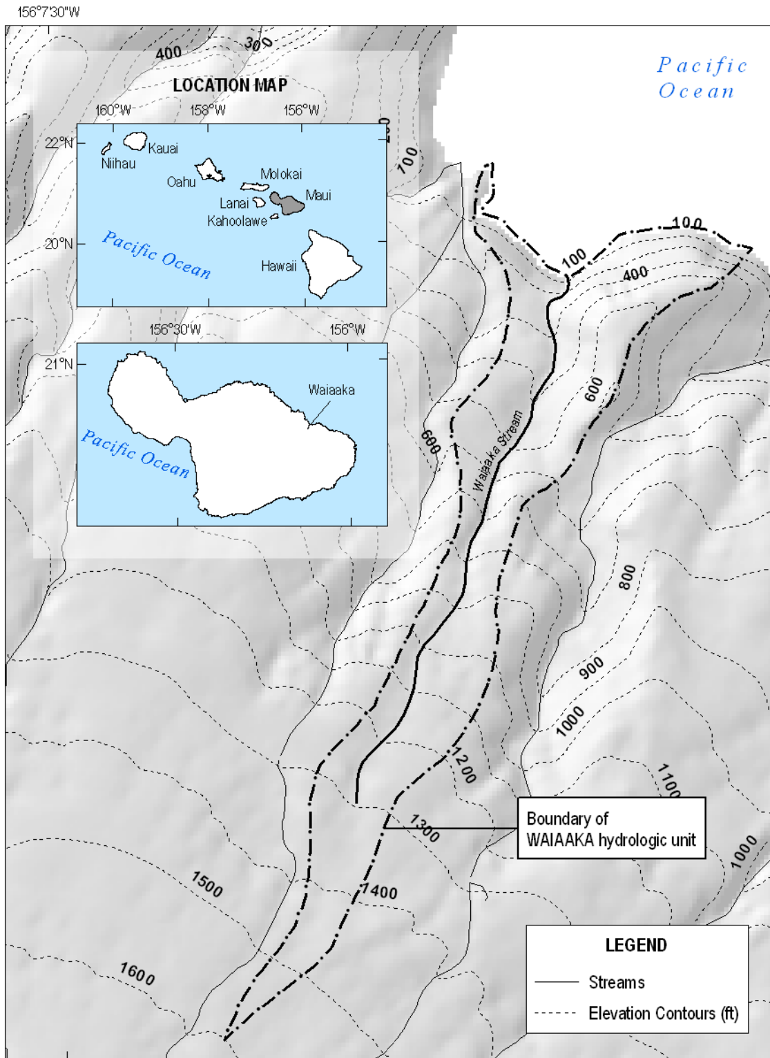
Figure 1-4. Elevation range and the location of Waiiaka hydrologic unit. (Source: State of Hawaii, Office of Planning, 1983; USGS, 2001b).
