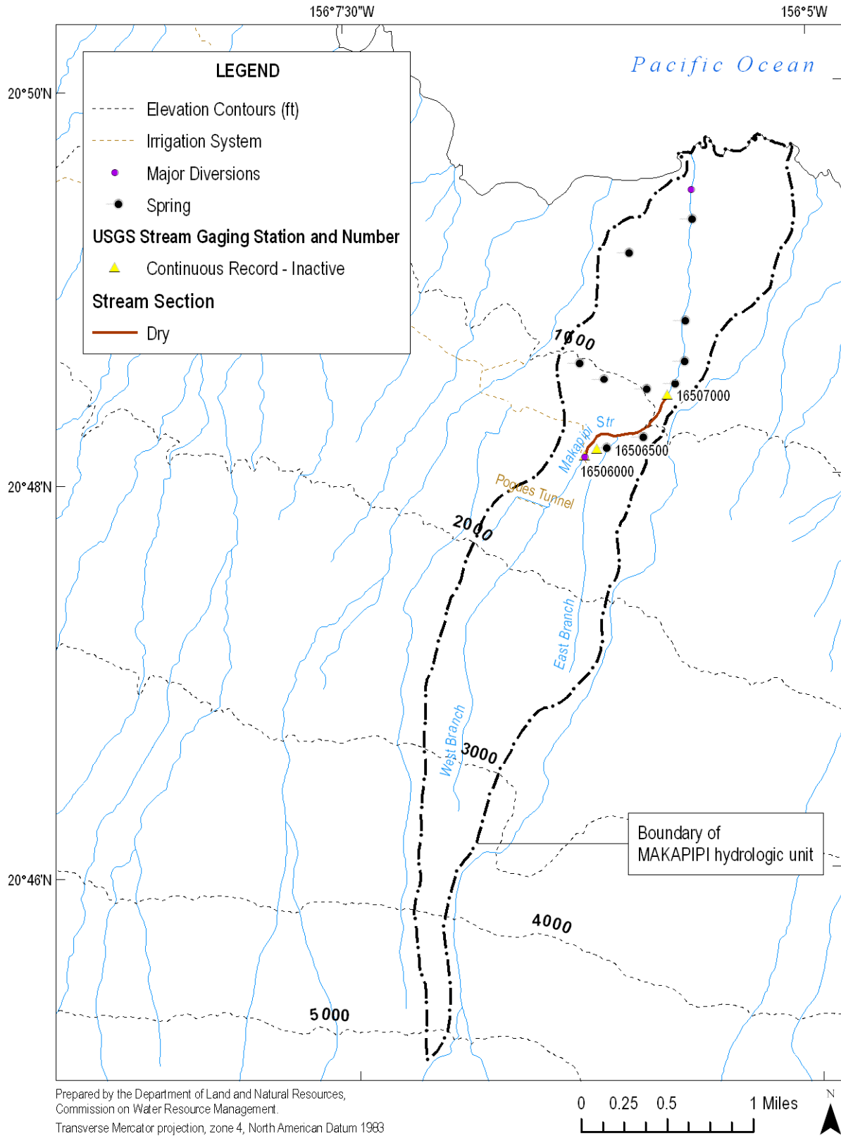
Figure 3-3. Location of diversions, irrigation systems, and USGS gaging stations in Makapii hydrologic unit (Source: State of Hawaii, Office of Planning, n.d.; 1996, 2004c; 2005; USGS, 2001b).
