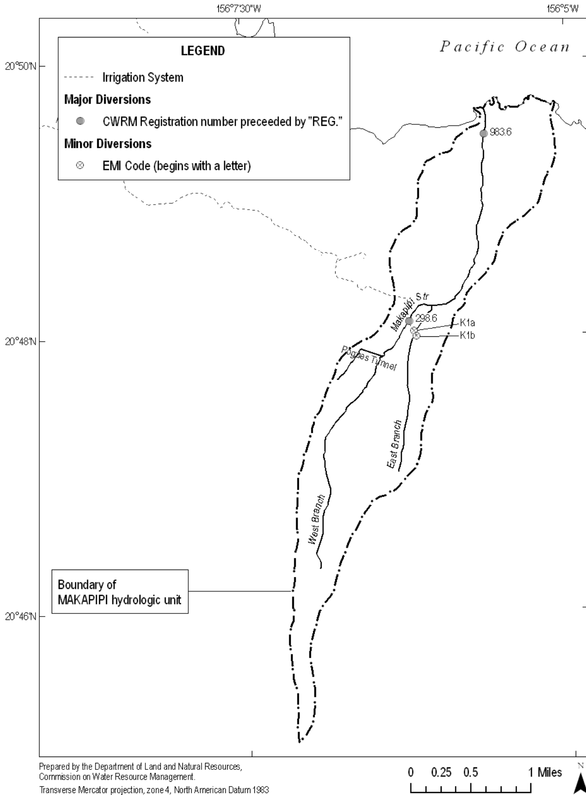
Figure 13-19. All registered diversions and EMI minor diversions identified in the Makapipi hydrologic unit (Source: East Maui Irrigation Company, 1970; State of Hawaii, Commission on Water Resource Management, 2008f; USGS, 2001b).
