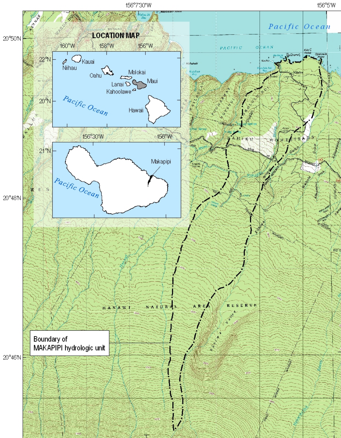
Figure 1-3. Topographic map of the Makapipi hydrologic unit in east Maui, Hawaii (Source: USGS, 1996).
