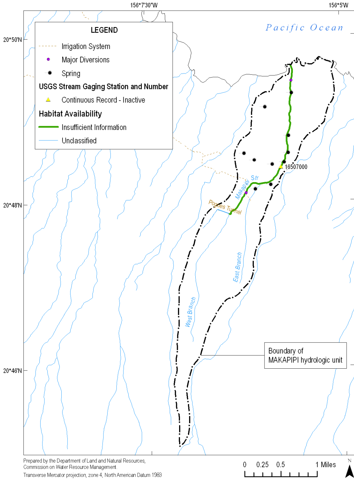
Figure 4-3. Estimated habitat availability in Makapipi hydrologic unit (Source: Gingerich and Wolff, 2005; USGS, 2001b).
