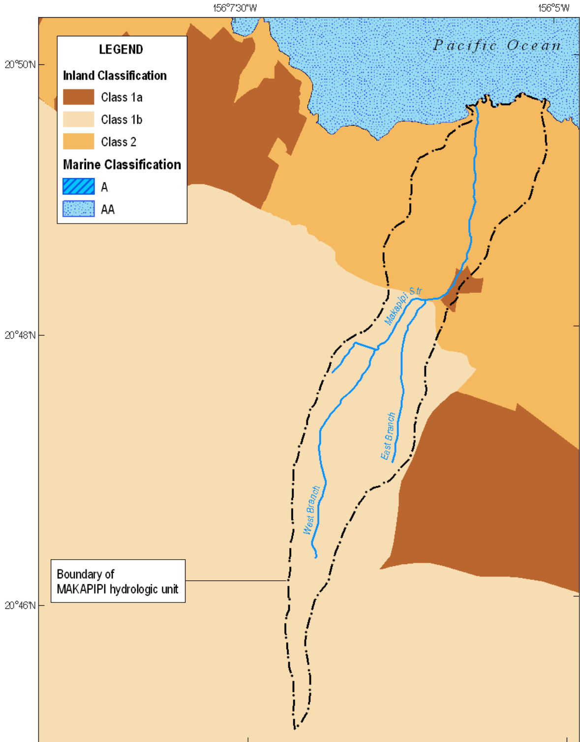
Figure 10-1. Water quality standards for the Makapipi hydrologic unit. (Source: State of Hawaii, Office of Planning, 2002e; 2008). The classifications are general in nature and should be used in conjunction with Hawaii Administrative Rules, Chapter 11-54, Water Quality Standards.
