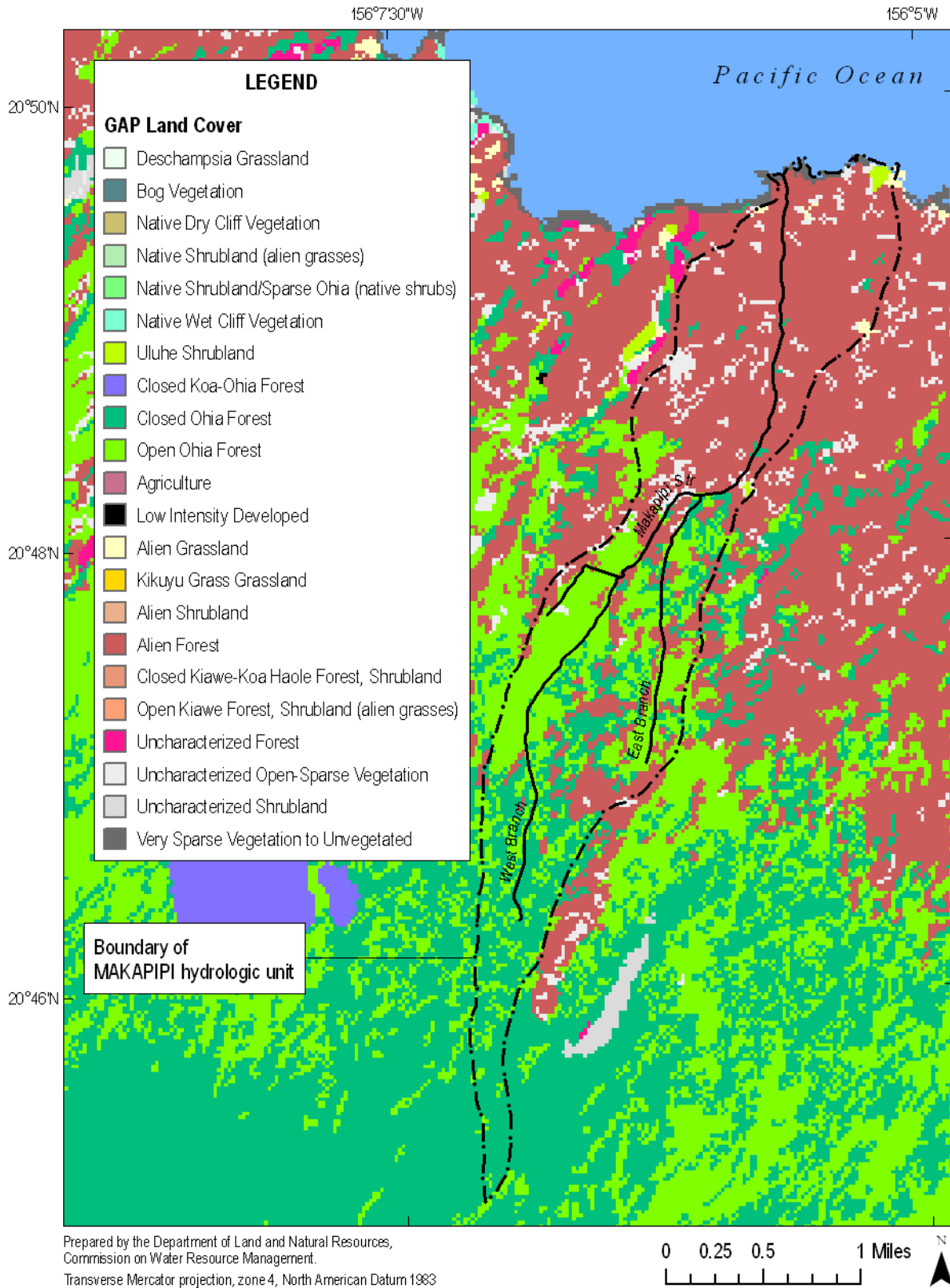
Figure 2-7. Hawaii GAP land cover classes in Makapipi hydrologic unit (Source: Hawaii GAP Analysis Program, 2005; USGS, 2001b).
