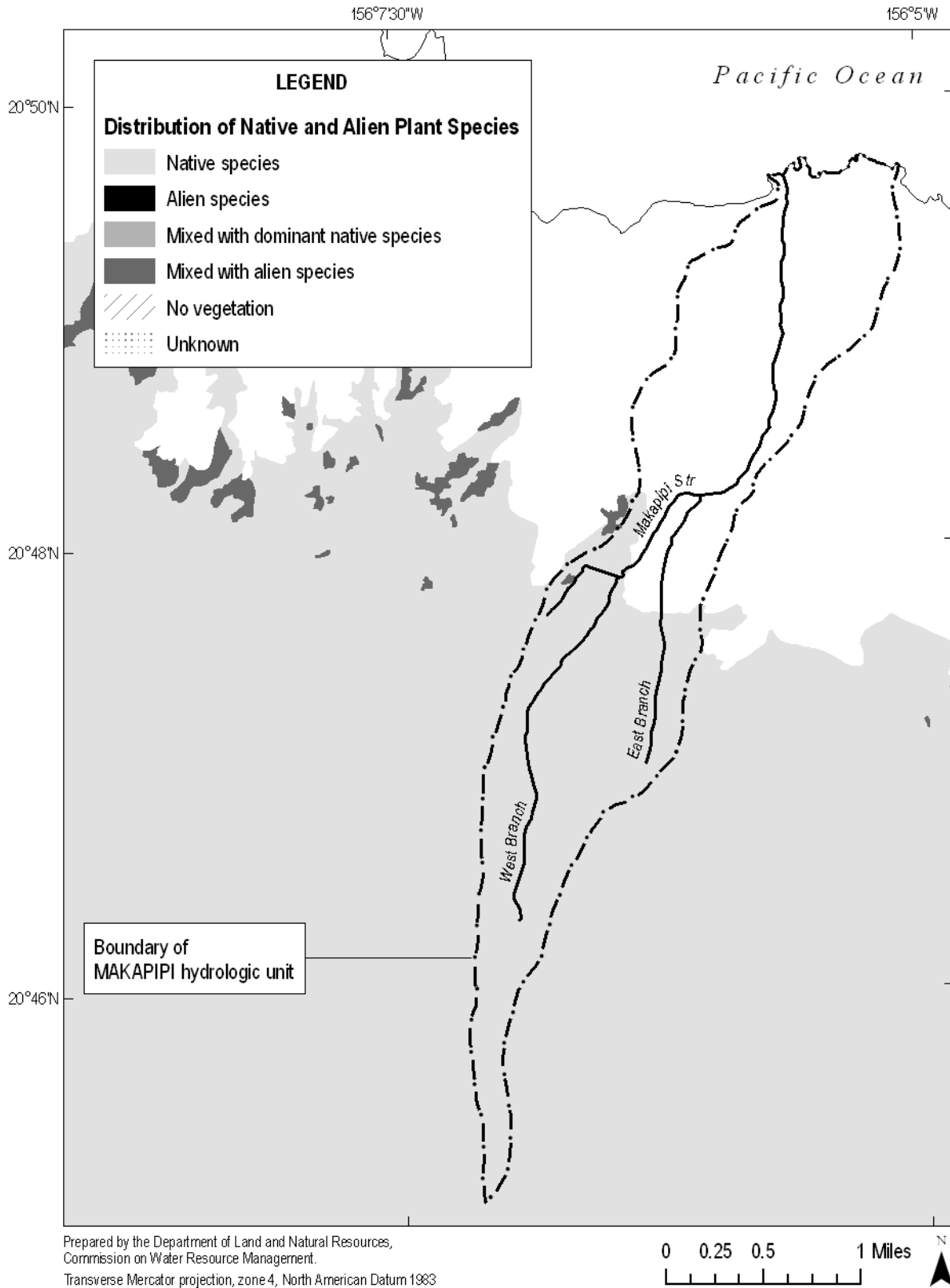
Figure 6-3. Distribution of native and alien plant species for Makapii hydrologic unit (Source: Jacobi, 1989; Scott et al., 1986; State of Hawaii, Office of Planning, 1992, 2004b; 2004d; USGS, 2001b).
