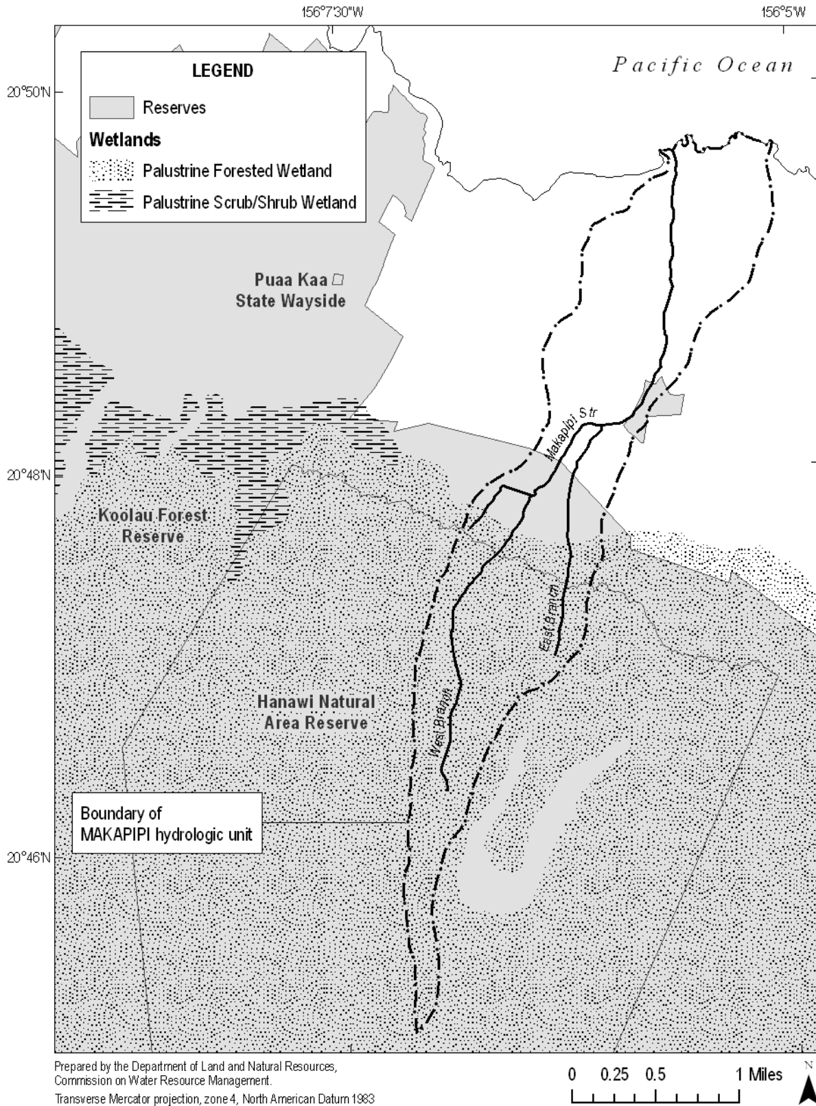
Figure 6-2. Reserves and wetlands for the Makapipi hydrologic unit (Source: State of Hawaii, Office of Planning, 2003; 2007b; USGS, 2001b).
