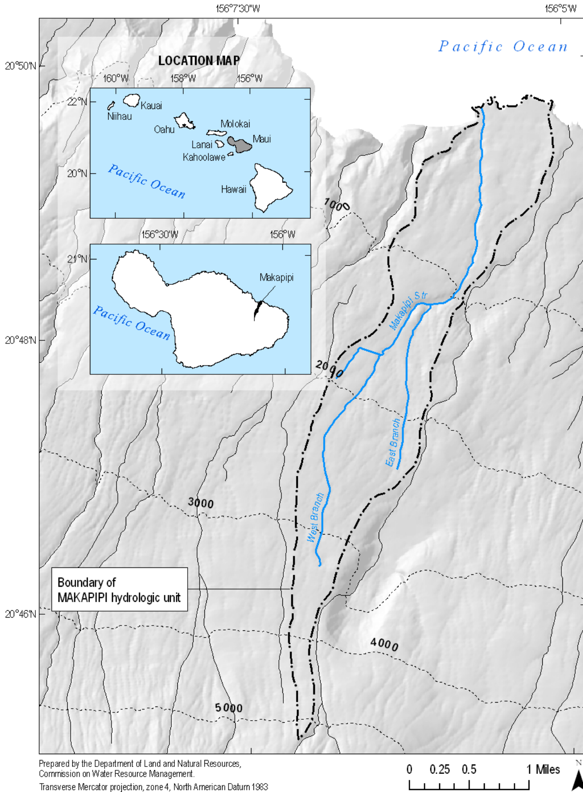
Figure 1-4. Elevation range and the location of Makapipi hydrologic unit. (Source: State of Hawaii, Office of Planning, 1983; USGS, 2001b).
