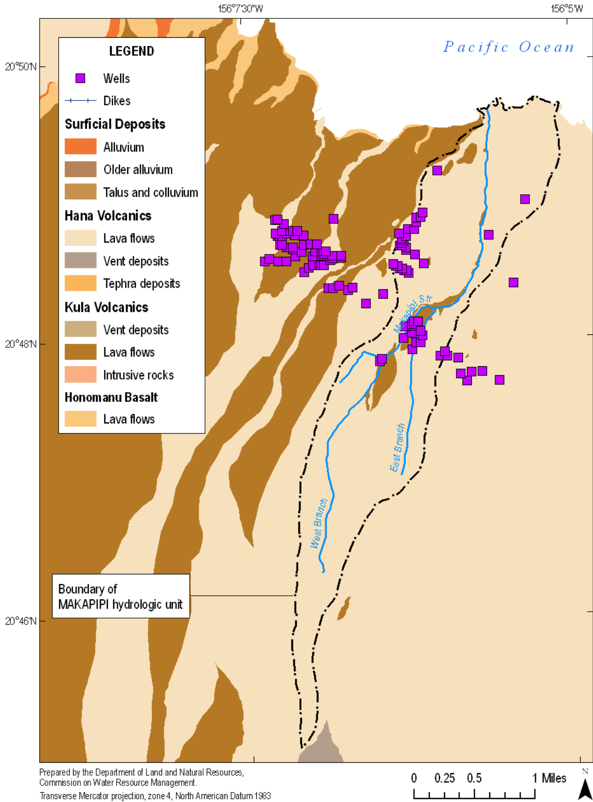
Figure 2-2. Generalized geology of Makapipi hydrologic unit (Source: Sherrod et al., 2007; State of Hawaii, Office of Planning, 2006a, and State of Hawaii, Commission on Water Resource Management, 2008d; USGS, 2001b).
