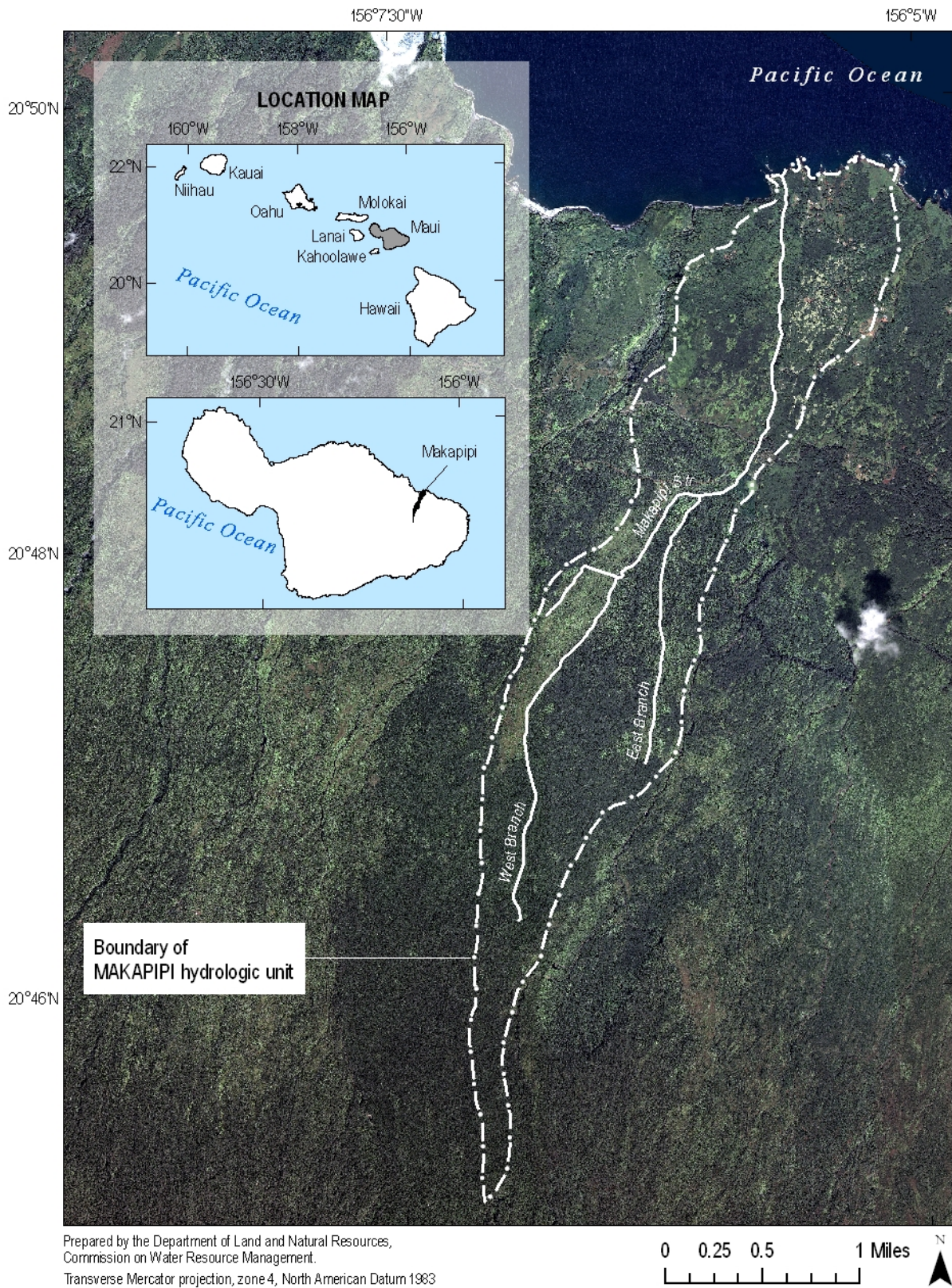
Figure 1-6. Quickbird satellite imagery of Makapipi hydrologic unit (Source: County of Maui, Planning Department, 2004; USGS, 2001b).
