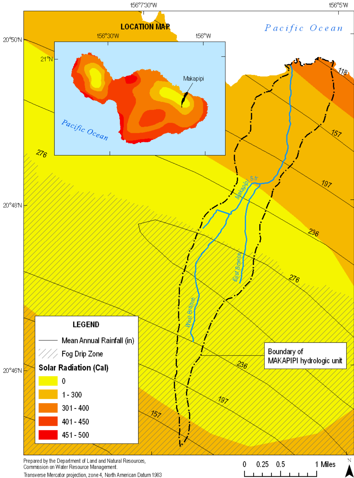
Figure 2-4. Mean annual rainfall and fog area in Makapipi; and solar radiation for Makapipi and the island of Maui, Hawaii (Source: Giambelluca et al., 1986; State of Hawaii, Office of Planning, 2006b; 2006c; USGS, 2001b).
