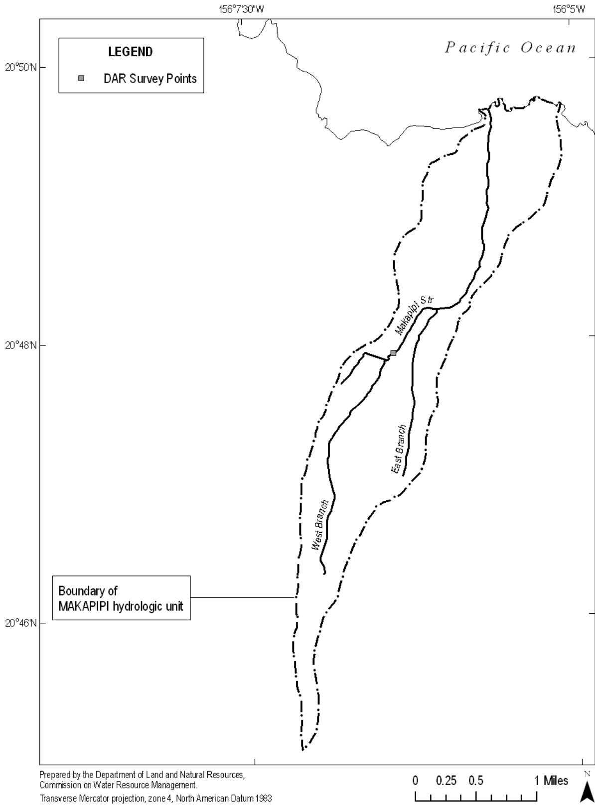
Figure 4-4. Division of Aquatic Resource survey point in Makapii Stream (Source: DAR, 2009).
