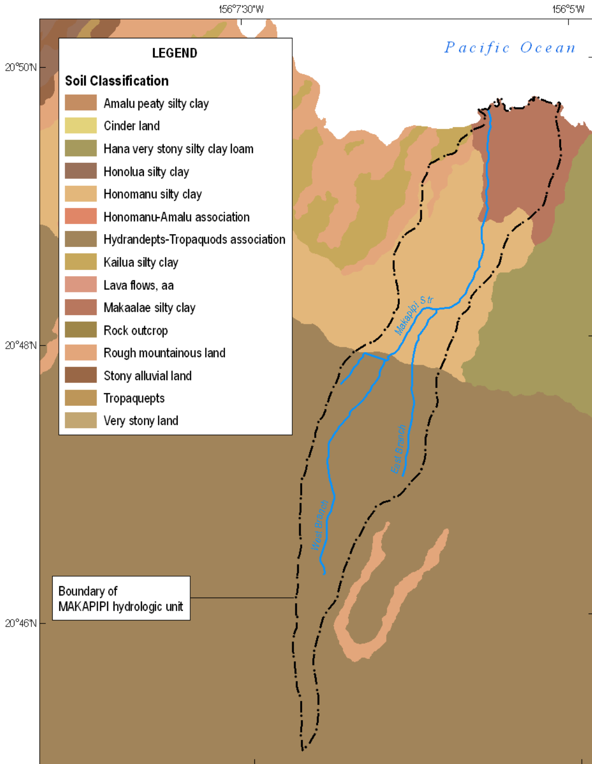
Figure 2-3. Soil classification in Makapii hydrologic unit (Source: State of Hawaii, Office of Planning, 2007c; USGS, 2001b).
