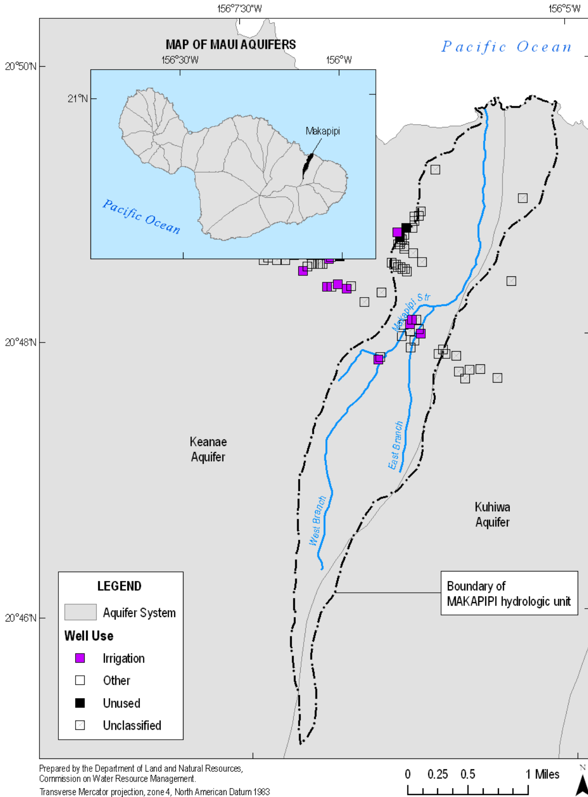
Figure 3-2. Aquifer system area and well locations in Makapipi hydrologic unit (Source: State of Hawaii, Office of Planning, 2006b; State of Hawaii, Commission on Water Resource Management, 2008d; USGS, 2001b).
