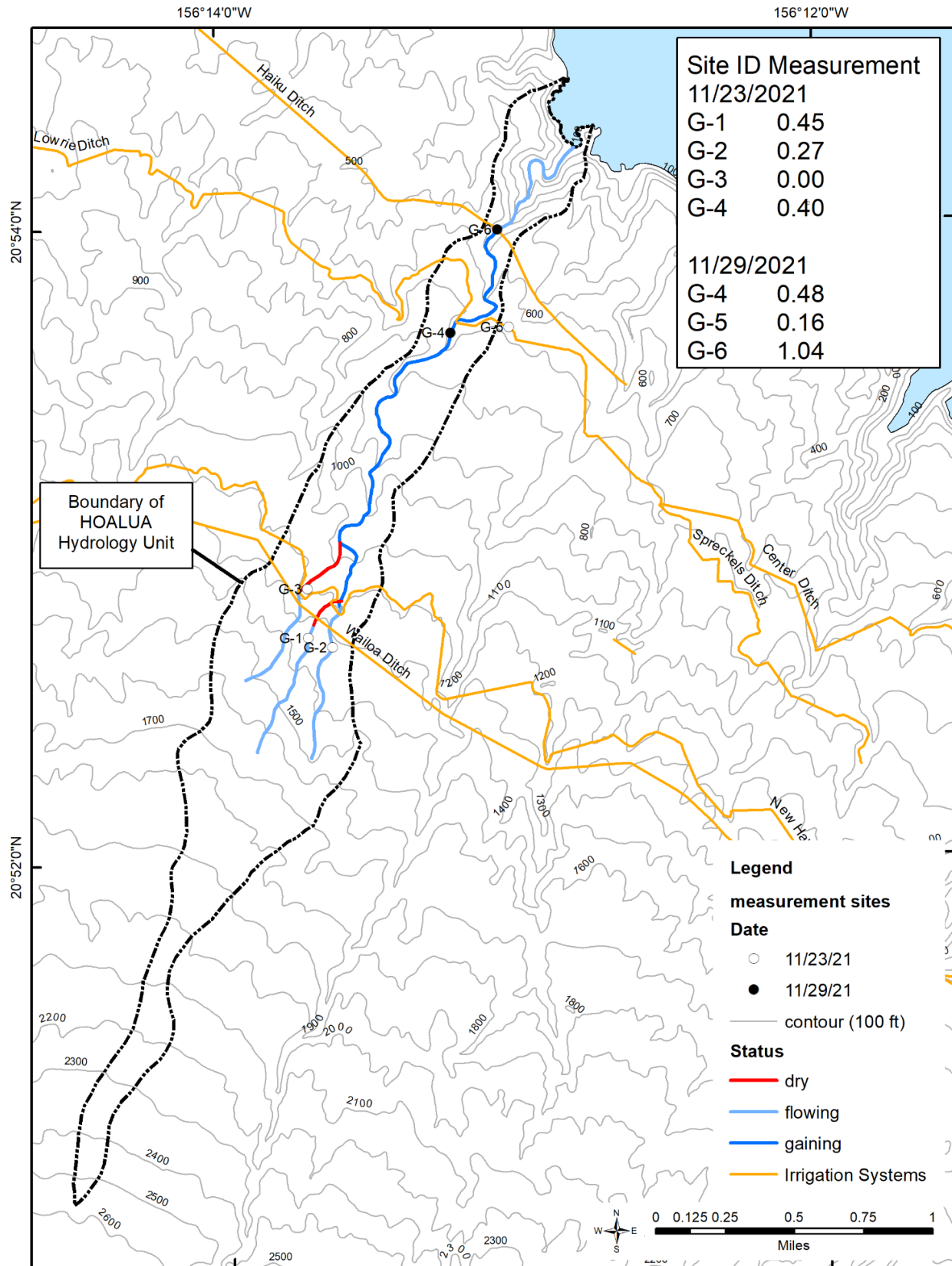
Figure 3-5. Seepage run results for Hoalua Stream in East Maui, Hawai'i.
