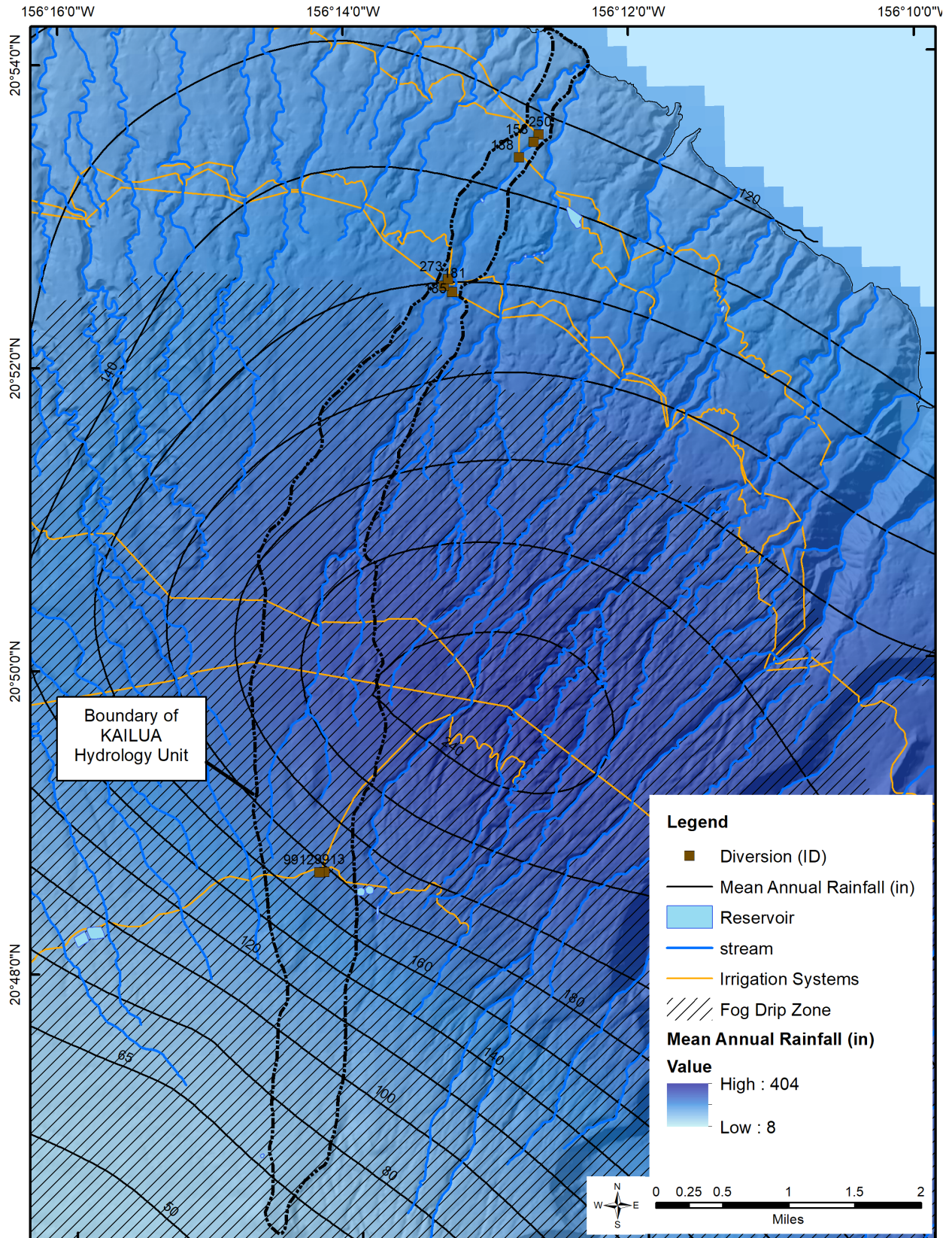
Figure 2-4. Mean annual rainfall and generalized fog drip zone in the Kailua hydrologic unit, Maui. (Source: Giambelluca et al., 2013)
