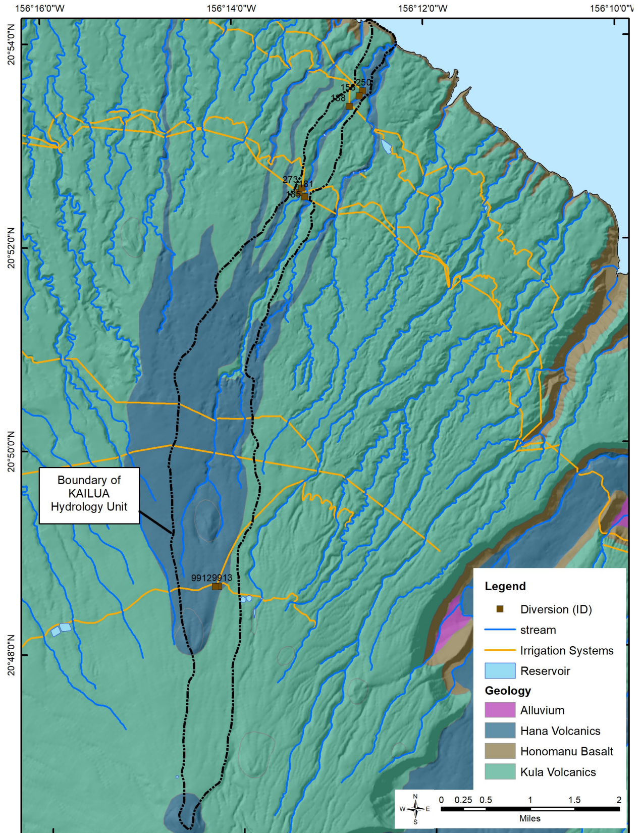
Figure 2-1. Generalized geology of the Kailua hydrologic unit, Maui. (Source: Sherrod et al., 2007)
