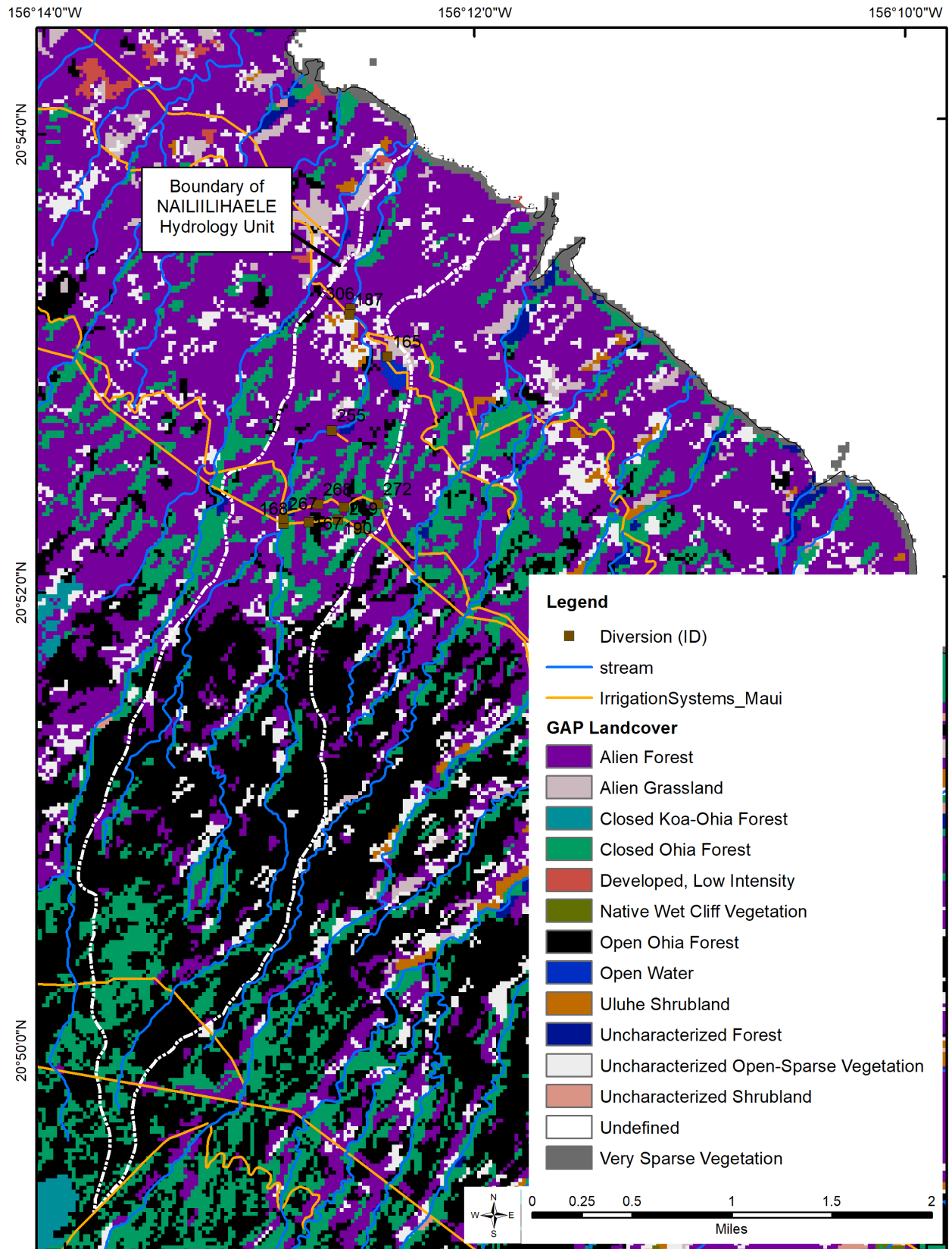
Figure 2-9. Hawaii GAP land cover classes of the Naililihaele hydrologic unit, Maui. (Source: USGS, 2001).
