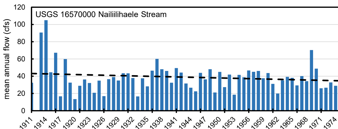
Figure 3-3. Mean annual flow in Nailiilihaele Stream at USGS station 16570000 from 1911 to 1975. (Source: USGS, 2020)
