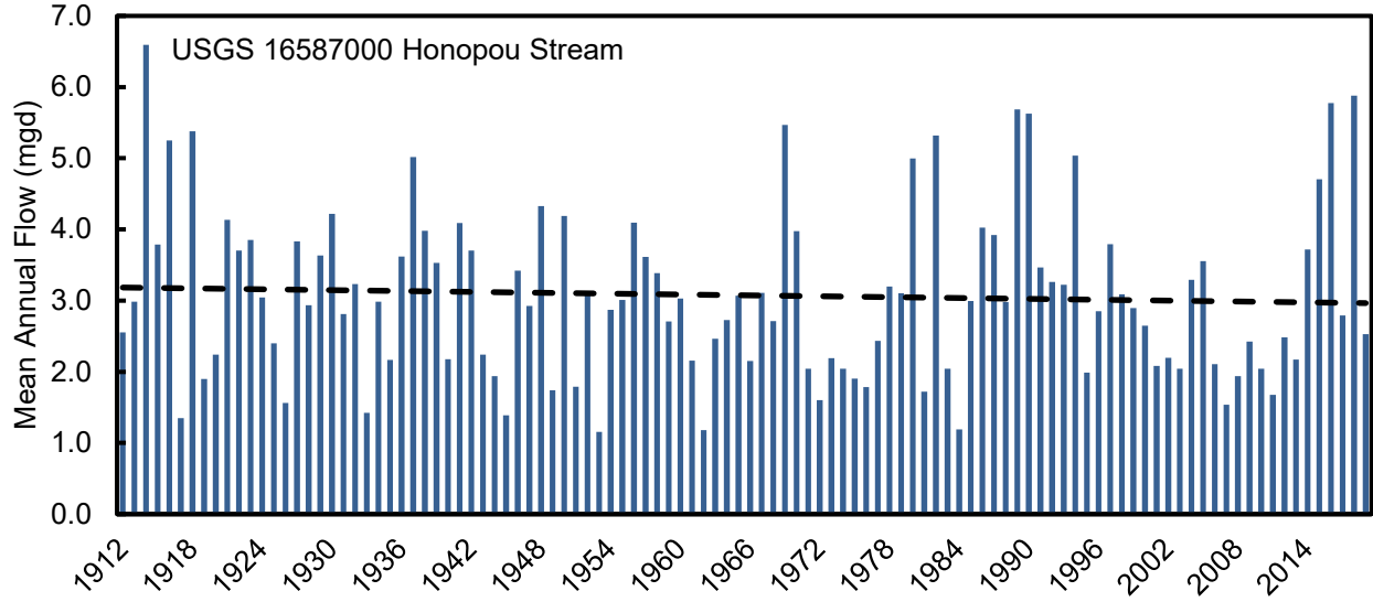
Figure 3-8. Mean annual flow (million gallons per day, mgd) at USGS station 16587000 on Honopou Stream, Maui. Line represents linear regression trend over the period of record. (Source: USGS, 2020)
