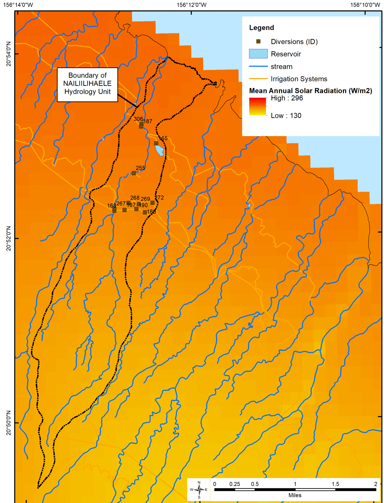
Figure 2-5. Mean annual solar radiation of the Naililihaele hydrologic unit, Maui. (Source: State of Hawaii, Office of Planning, 2015c)
