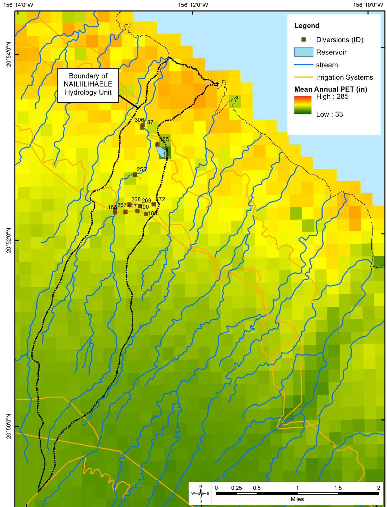
Figure 2-6. Mean annual potential evapotranspiration (Penman-Monteith method) of the Naililihaele hydrologic unit, Maui. (Source: Giambelluca et al., 2014)
