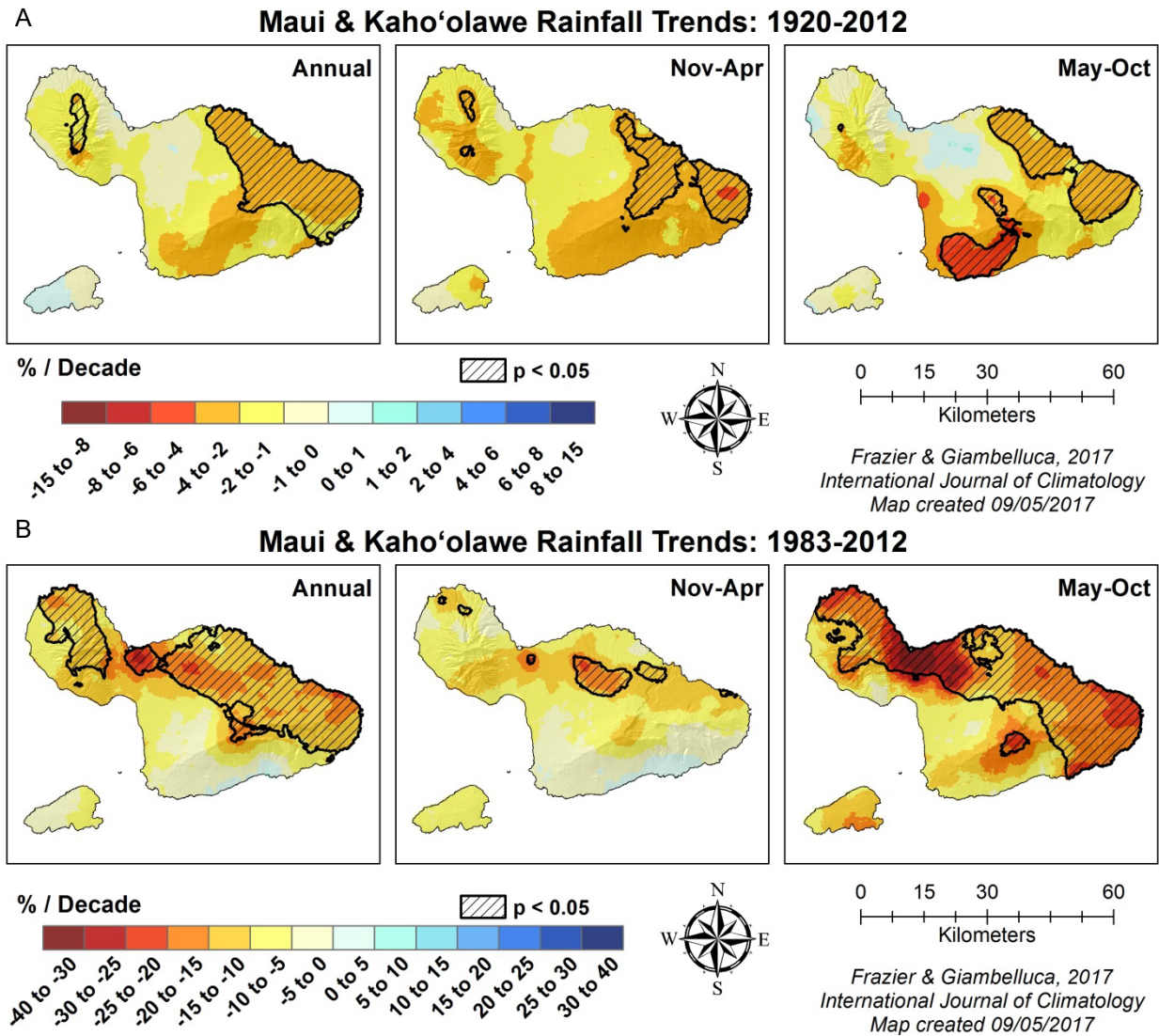
Figure 3-6. Annual, wet season (Nov-Apr) and dry season (May-Oct) rainfall trends for the 1920-2012 (A) and 1983-2012 (B) periods, Maui. Hashed line areas represent significant trend over the period. (with permission from Frazier and Giambelluca, 2017)
