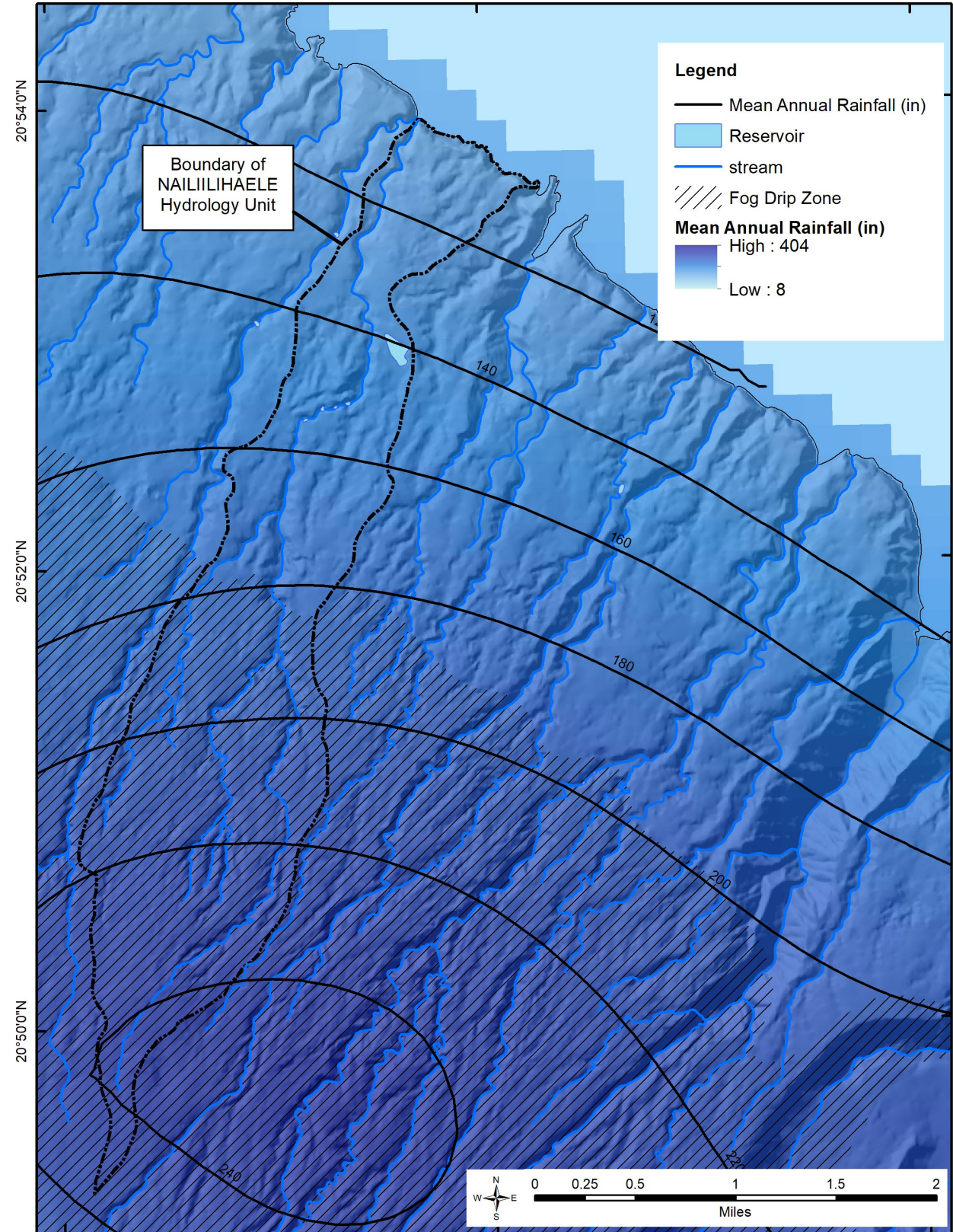
Figure 2-4. Mean annual rainfall and fog drip zone in the Naililihaele hydrologic unit, Maui. (Source: Giambelluca et al., 2013)
