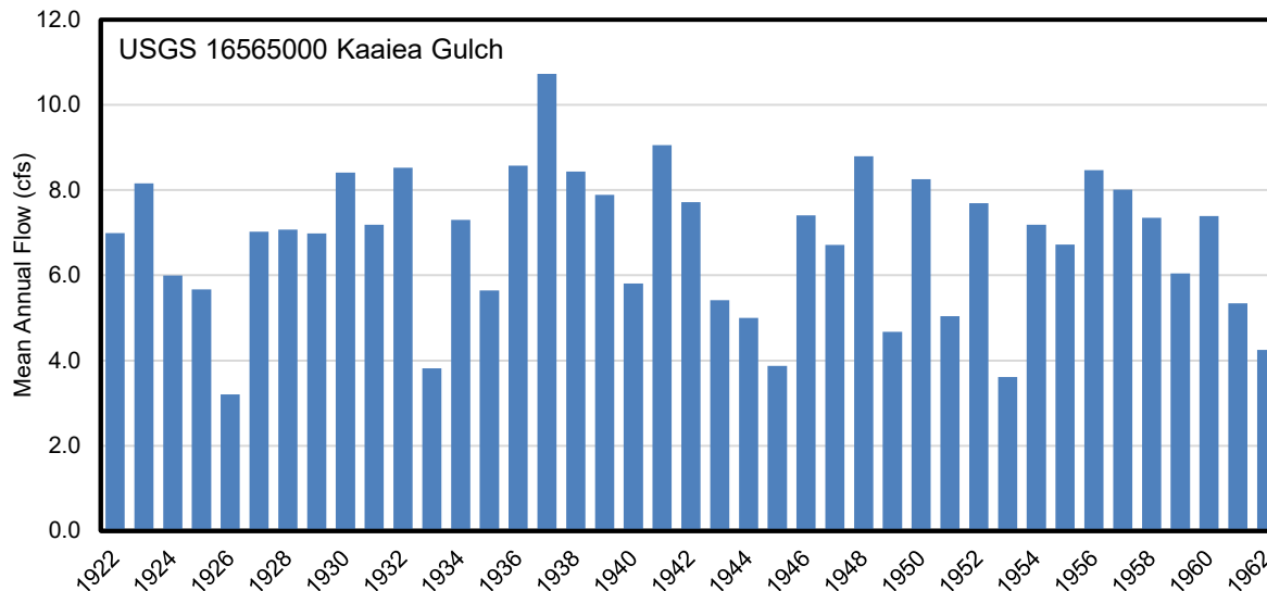
Figure 3-3. Mean annual flow in Kaaiea Stream at USGS station 16565000 from 1922 to 1962. (Source: USGS, 2020)
