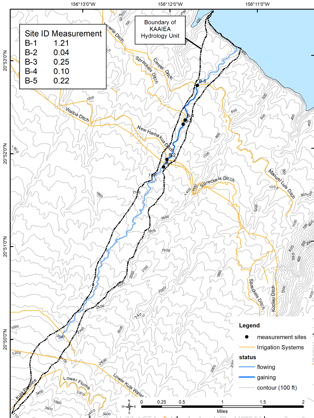
Figure 3-5. Seepage run results for the Kaaiea hydrologic unit, East Maui, Hawaii.
