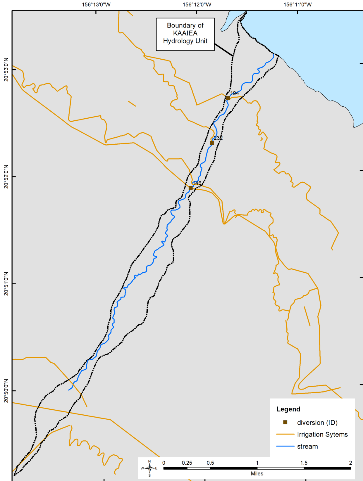
Figure 14-1. All registered diversions (ID) and ditches identified in the Kaaiea hydrologic unit, Maui. (Source: State of Hawaii, Commission on Water Resource Management, 2015g)
