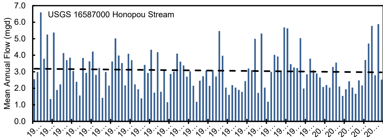
Figure 3-3. Mean annual flow (million gallons per day, mgd) at USGS station 16587000 on Honopou Stream, Maui. Line represents linear regression trend over the period of record. (Source: USGS, 2020)
