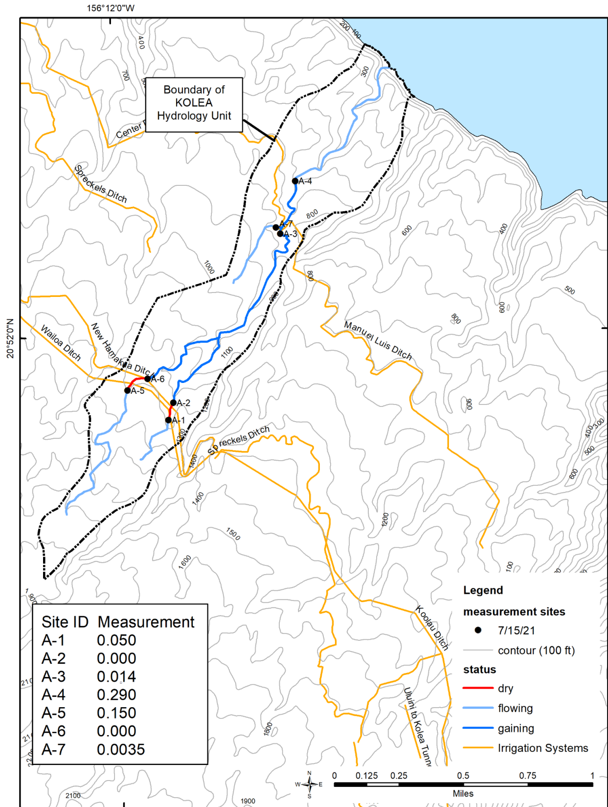
Figure 3-5. Seepage run results for the Kolea hydrologic unit, East Maui, Hawaii.
