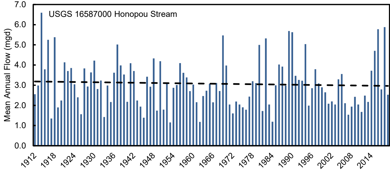
Figure 3-6. Mean annual flow (million gallons per day, mgd) at USGS station 16587000 on Honopou Stream, Maui. Line represents linear regression trend over the period of record. (Source: USGS, 2020)
